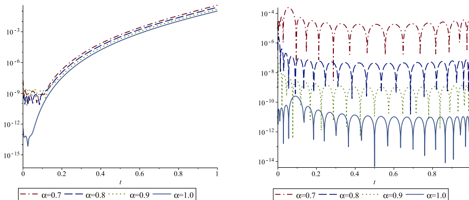
(a) Graph of the residual errors using the Tau methods
