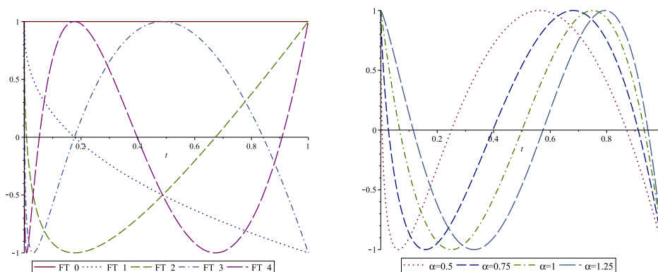
(a) Graph of the FCFs with \alpha = 0.40 and various values of n (b) Graph of the FCFs with n = 4 and various values of \alpha
